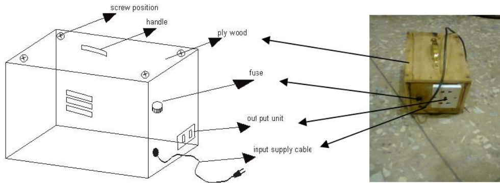
Fig. 3b. Back view of the cased transformer
