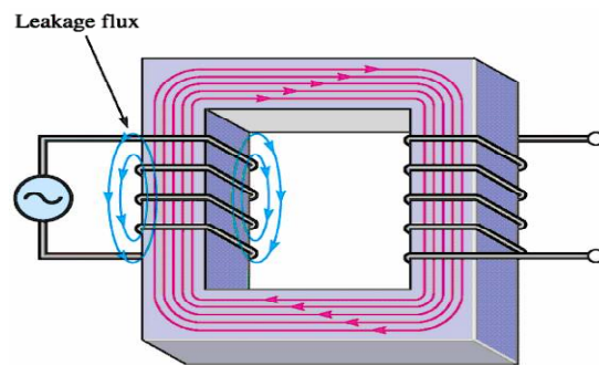
Fig. 1. Primary and secondary winding (Prof. Andrew H A 2004)
