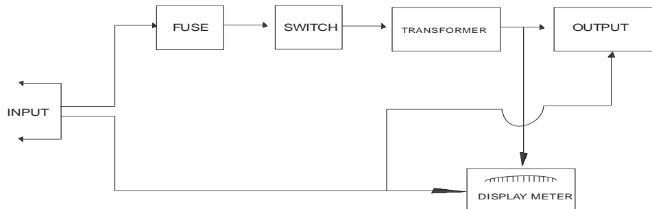
Fig. 2. Circuit diagram of the constructed device
