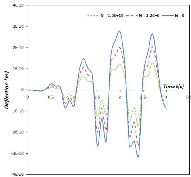
Fig. 24. The deflection profile of the moving mass system's fixed-fixed non-uniform damped Rayleigh beam under the influence of a harmonic moving load for different axial force values
