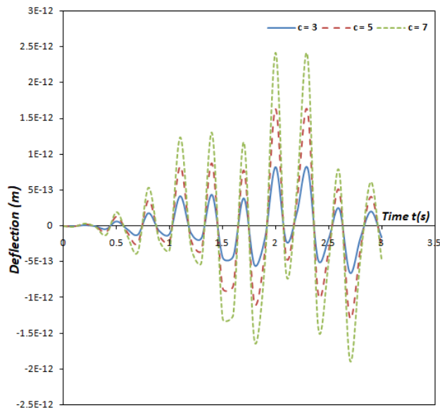
Fig. 26. The deflection profile of the moving mass system's fixed-free non-uniform damped Rayleigh beam under the influence of a harmonic moving load for different speed values
