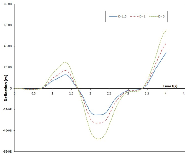
Fig. 6. The deflection profile of the moving mass system’s pinned-pinned non-uniform damped Rayleigh beam under the influence of a harmonic moving load for different mass ratio values
