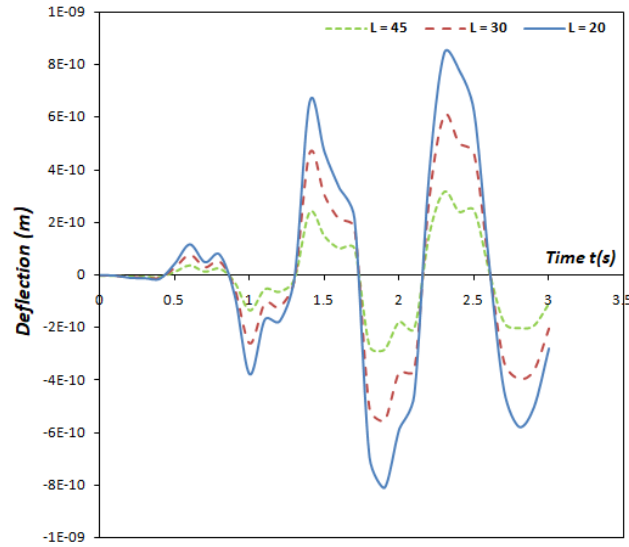
Fig. 15. The deflection profile of the moving force system's fixed-fixed non-uniform damped Rayleigh beam under the influence of a harmonic moving load for different Lenght values
