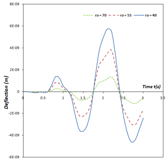
Fig. 21. The deflection profile of the moving force system’s fixed-fixed non-uniform damped Rayleigh beam under the influence of a harmonic moving load for different rotatory inertia values
