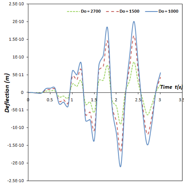
Fig. 20. The deflection profile of the moving mass system's fixed-fixed non-uniform damped Rayleigh beam under the influence of a harmonic moving load for different damping coefficient values
