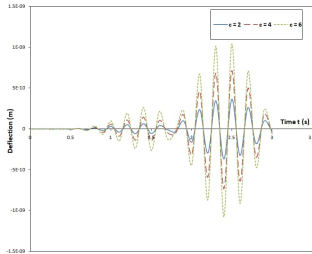
Fig. 2. The deflection profile of the moving mass system’s pinned-pinned non-uniform damped Rayleigh beam under the influence of a harmonic moving load for different speed values
