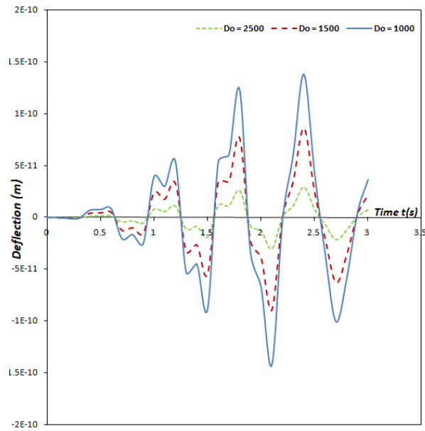
Fig. 19. The deflection profile of the moving force system's fixed-fixed non-uniform damped Rayleigh beam under the influence of a harmonic moving load for different damping coefficient values
