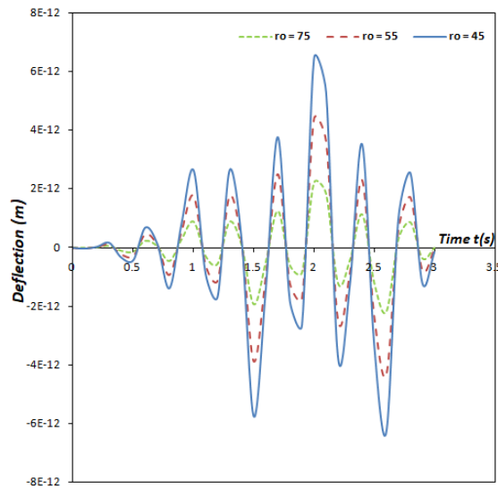
Fig. 34. The deflection profile of the moving mass system’s fixed-free non-uniform damped Rayleigh beam under the influence of a harmonic moving load for different rotatory inertia values
