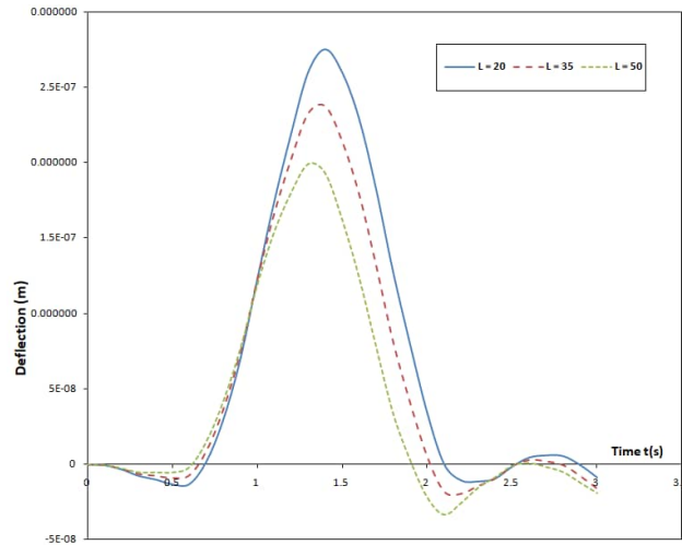
Fig. 3. The deflection profile of the moving force system's pinned-pinned non-uniform damped Rayleigh beam under the influence of a harmonic moving load for different Length values
