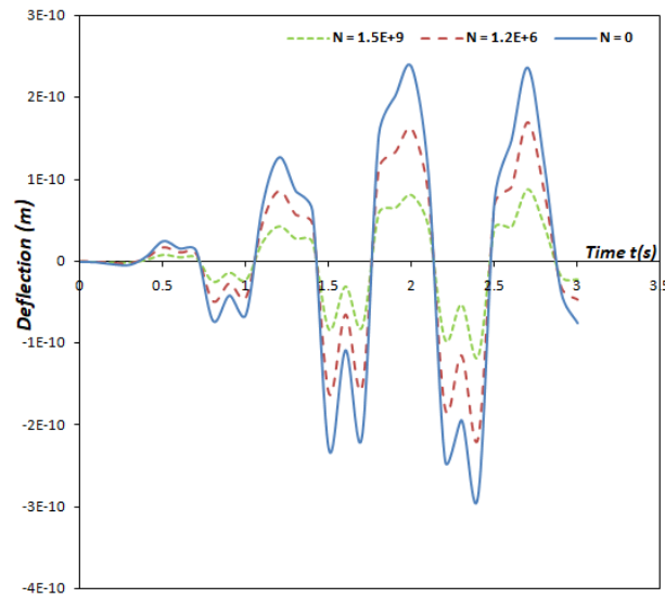
Fig. 23. The deflection profile of the moving force system's fixed-fixed non-uniform damped Rayleigh beam under the influence of a harmonic moving load for different axial force values
