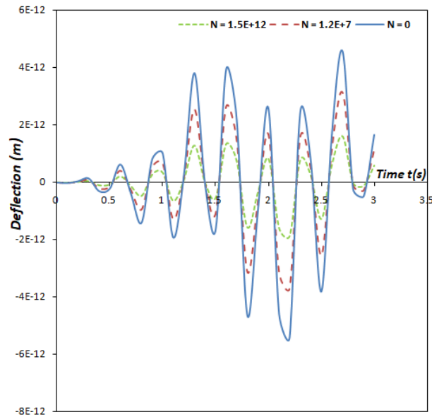
Fig. 36. The deflection profile of the moving mass system's fixed-free non-uniform damped Rayleigh beam under the influence of a harmonic moving load for different axial force values
