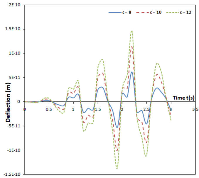
Fig. 14. The deflection profile of the moving mass system's fixed-fixed non-uniform damped Rayleigh beam under the influence of a harmonic moving load for different speed values
