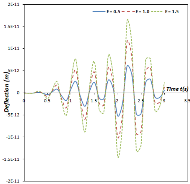
Fig. 18. The deflection profile of the moving mass system's fixed-fixed non-uniform damped Rayleigh beam under the influence of a harmonic moving load for different mass ratio values
