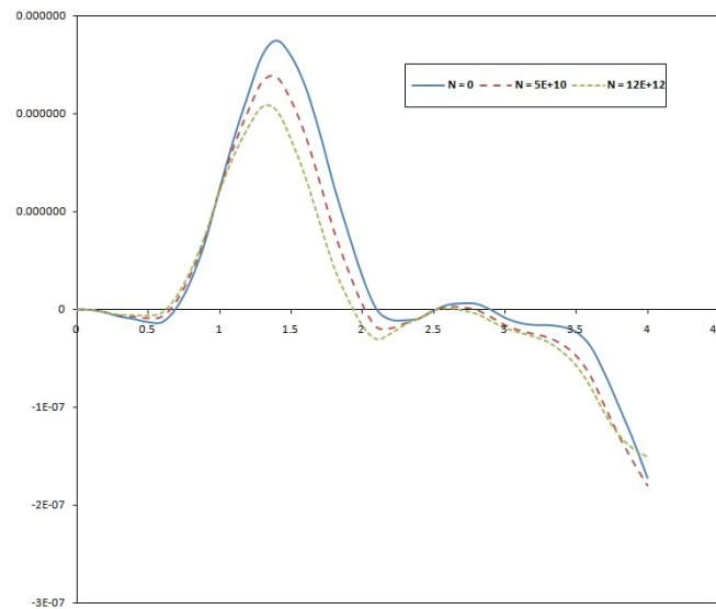
Fig. 12. The deflection profile of the moving mass system's pinned-pinned non-uniform damped Rayleigh beam under the influence of a harmonic moving load for different axial force values
