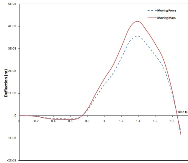
Fig. 37. Transverse deflection of the non-uniform damped Rayleigh beam for moving force and moving mass
