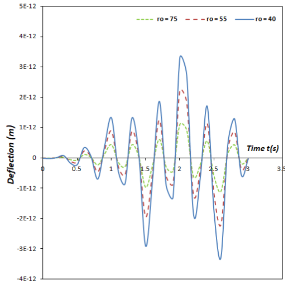
Fig. 33. The deflection profile of the moving force system’s fixed-free non-uniform damped Rayleigh beam under the influence of a harmonic moving load for different rotatory inertia values
