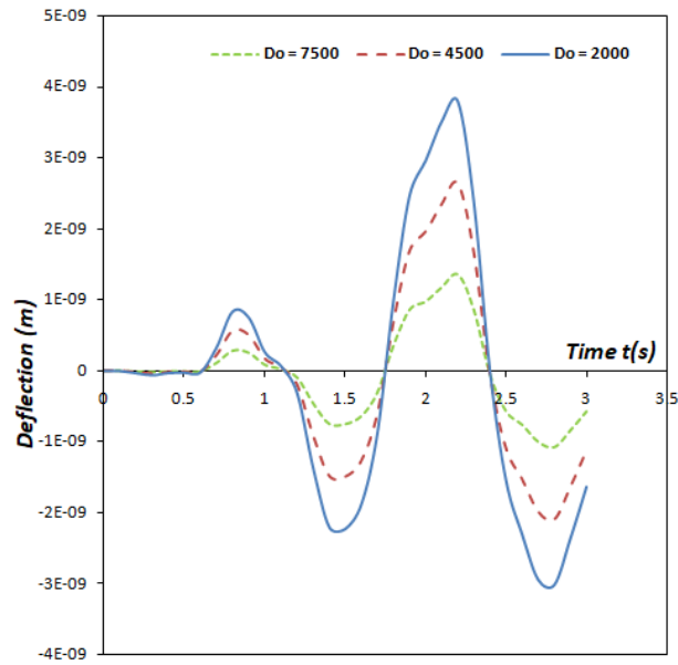
Fig. 31. The deflection profile of the moving force system's fixed-free non-uniform damped Rayleigh beam under the influence of a harmonic moving load for different damping coefficient values
