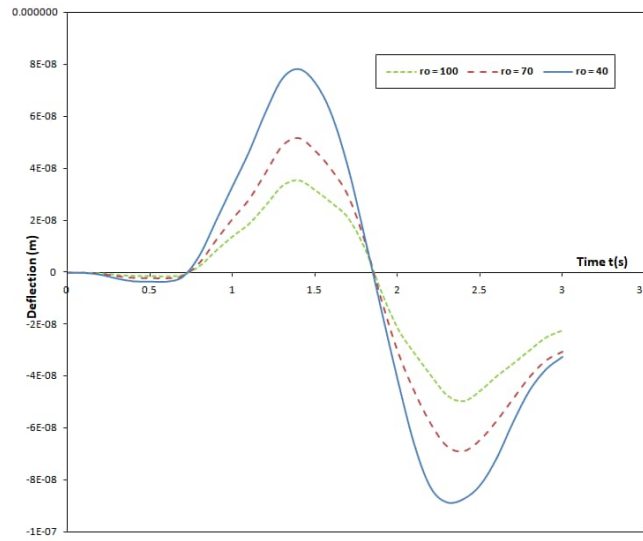
Fig. 9. The deflection profile of the moving force system's pinned-pinned non-uniform damped Rayleigh beam under the influence of a harmonic moving load for different rotatory inertia values
