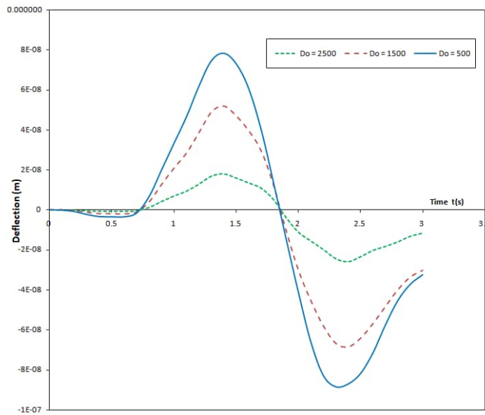
Fig. 8. The deflection profile of the moving mass system’s pinned-pinned non-uniform damped Rayleigh beam under the influence of a harmonic moving load for different damping coefficient values
