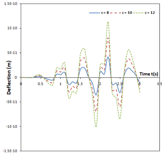
Fig. 13. The deflection profile of the moving force system's fixed-fixed non-uniform damped Rayleigh beam under the influence of a harmonic moving load for different speed values
