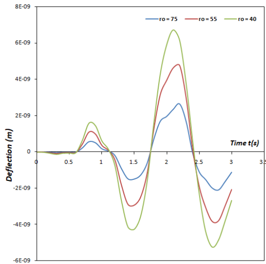
Fig. 22. The deflection profile of the moving mass system’s fixed-fixed non-uniform damped Rayleigh beam under the influence of a harmonic moving load for different rotatory inertia values
