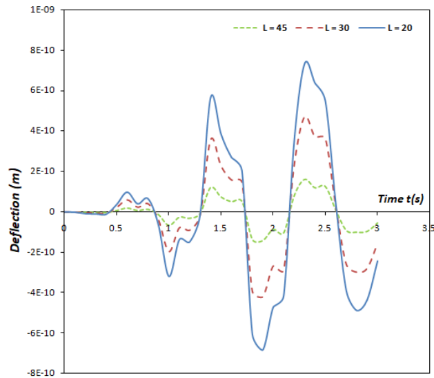
Fig. 16. The deflection profile of the moving mass system's fixed-fixed non-uniform damped Rayleigh beam under the influence of a harmonic moving load for different Lenght values
