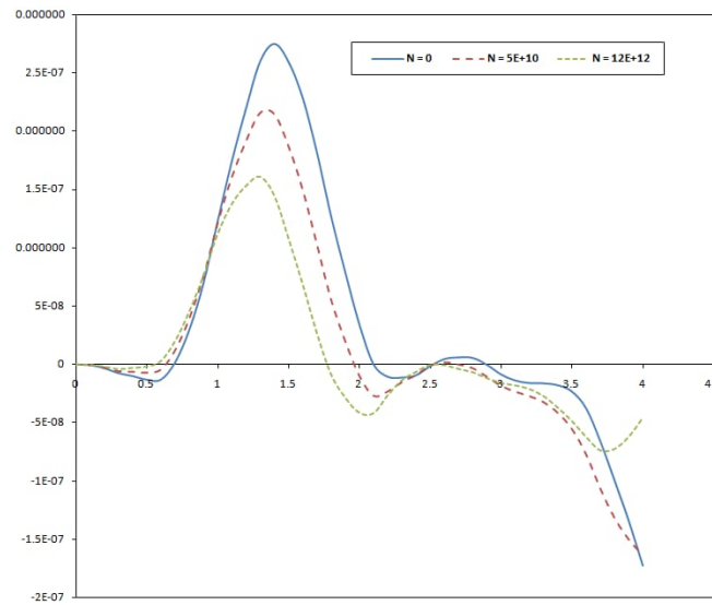
Fig. 11. The deflection profile of the moving force system's pinned-pinned non-uniform damped Rayleigh beam under the influence of a harmonic moving load for different axial force values
