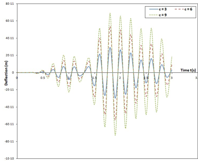
Fig. 1. The deflection profile of the moving force system’s pinned-pinned non-uniform damped Rayleigh beam under the influence of a harmonic moving load for different speed values
