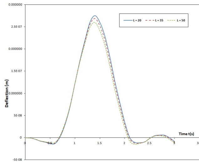
Fig. 4. The deflection profile of the moving mass system's pinned-pinned non-uniform damped Rayleigh beam under the influence of a harmonic moving load for different Length values
