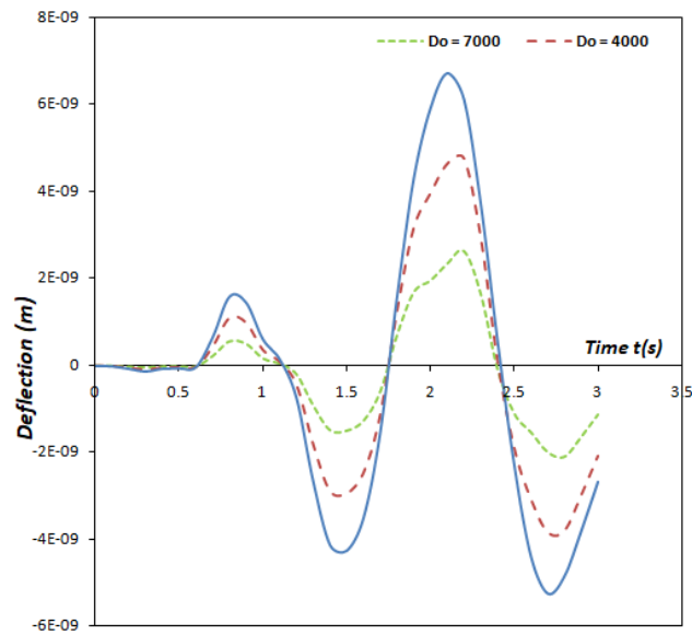
Fig. 32. The deflection profile of the moving mass system's fixed-free non-uniform damped Rayleigh beam under the influence of a harmonic moving load for different damping coefficient values
