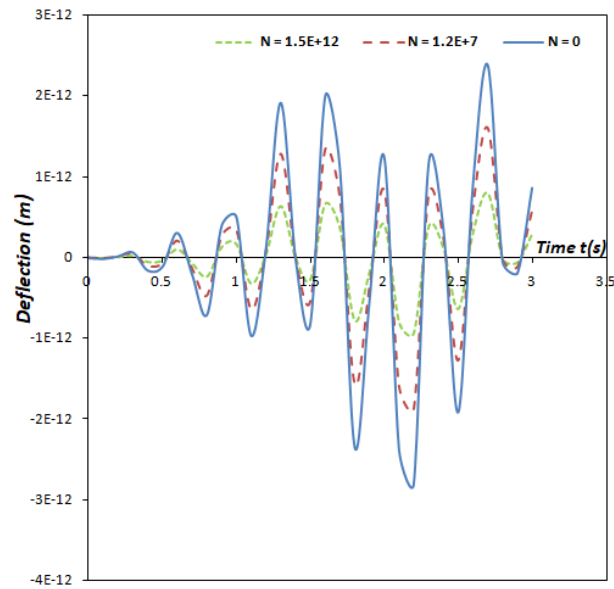
Fig. 35. The deflection profile of the moving force system's fixed-free non-uniform damped Rayleigh beam under the influence of a harmonic moving load for different axial force values
