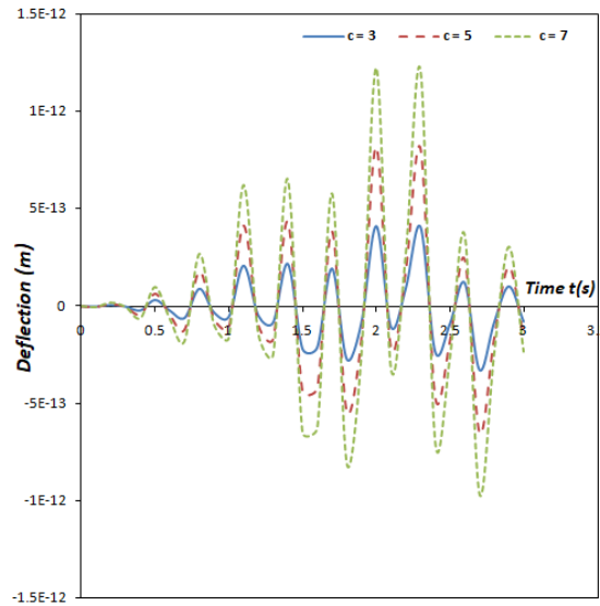
Fig. 25. The deflection profile of the moving force system's fixed-free non-uniform damped Rayleigh beam under the influence of a harmonic moving load for different speed values
