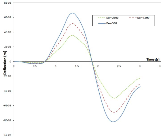
Fig. 7. The deflection profile of the moving force system’s pinned-pinned non-uniform damped Rayleigh beam under the influence of a harmonic moving load for different damping coefficient values
