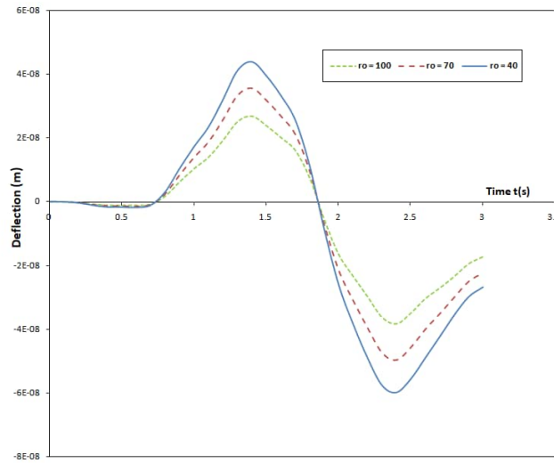
Fig. 10. The deflection profile of the moving mass system's pinned-pinned non-uniform damped Rayleigh beam under the influence of a harmonic moving load for different rotatory inertia values
