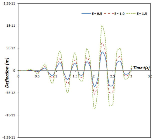
Fig. 17. The deflection profile of the moving force system's fixed-fixed non-uniform damped Rayleigh beam under the influence of a harmonic moving load for different mass ratio values
