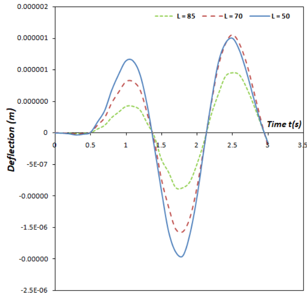
Fig. 27. The deflection profile of the moving force system’s fixed-free non-uniform damped Rayleigh beam under the influence of a harmonic moving load for different Length values
