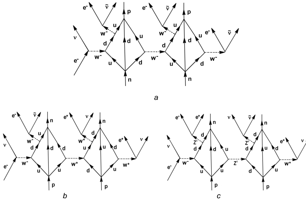
Fig. 3. Feynman diagrams for initiated (a) 2\beta^- - and (b, c) 2\beta^+ -decays
