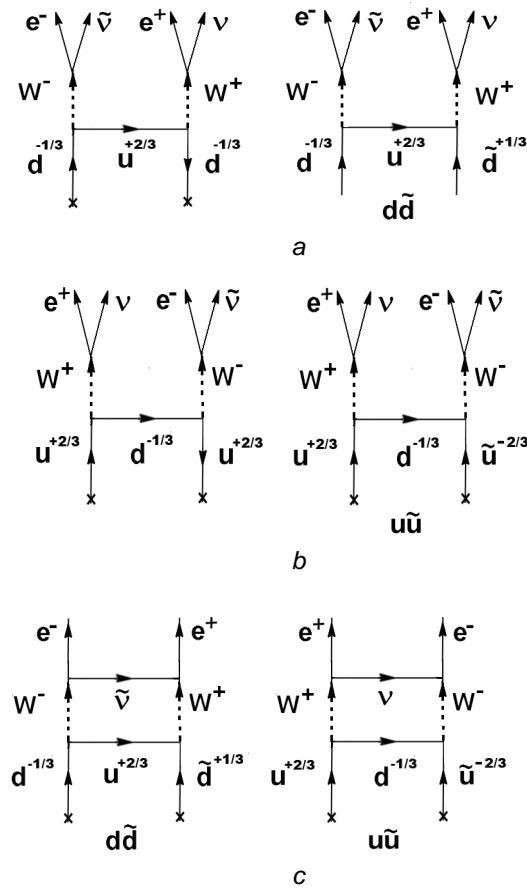
Fig. 4. Feynman diagrams for the formation of correlated e^-e^+ , e^-\tilde{\nu} и e^+\nu pairs initiated by the interaction between a \pi^0 -meson (quark-antiquark superposition d\bar{d} and u\bar{u} ) and the nucleons of the excited {}^8\text{Be}^* nucleus
