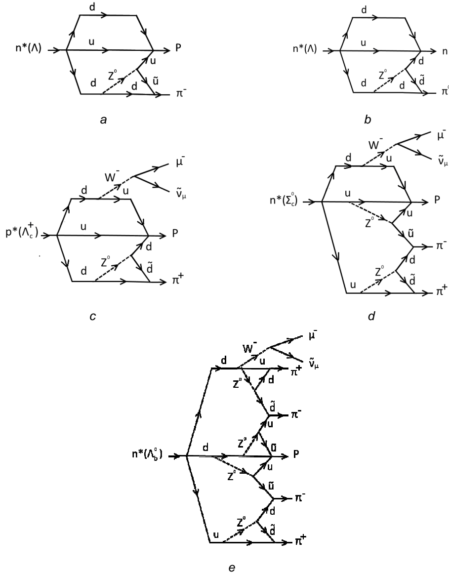
Fig. 2. Feynman diagrams for the decay of hyperons that contain (a, b) s -quark, (c, d) c -quark, and (e) b -quark
