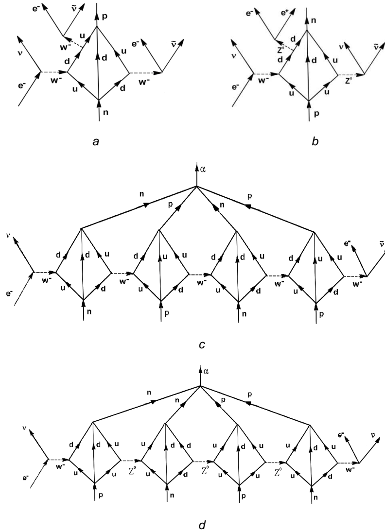
Fig. 1. Feynman diagrams for initiated (a) \beta^- -decays, (b) \beta^+ -decays, and (c, d) \alpha -decay
