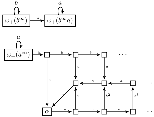
Fig. 4. Krieger graph G_K consisting of two separate weakly connected components (Proposition 4.1 (2)). The irreducible component containing the vertex \alpha := \omega_+((aba)^\infty) is the Fischer cover.
