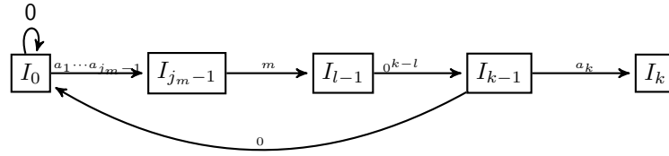
Fig. 2. The subgraph H of \mathcal{G}_\beta with 1_\beta = a_1a_2a_3\dots , where l := j_m + |m| .
