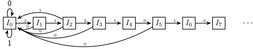
Fig. 1. Cover for the \beta -shift with 1_\beta = 2121010\dots
